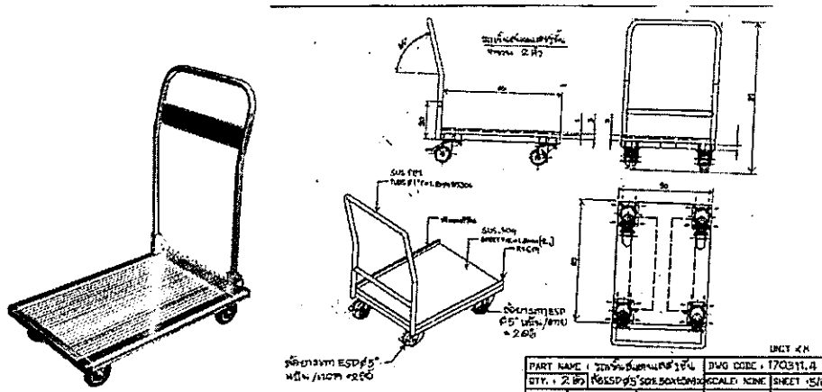
Figure 20: Example of single-tier stainless steel cart*
